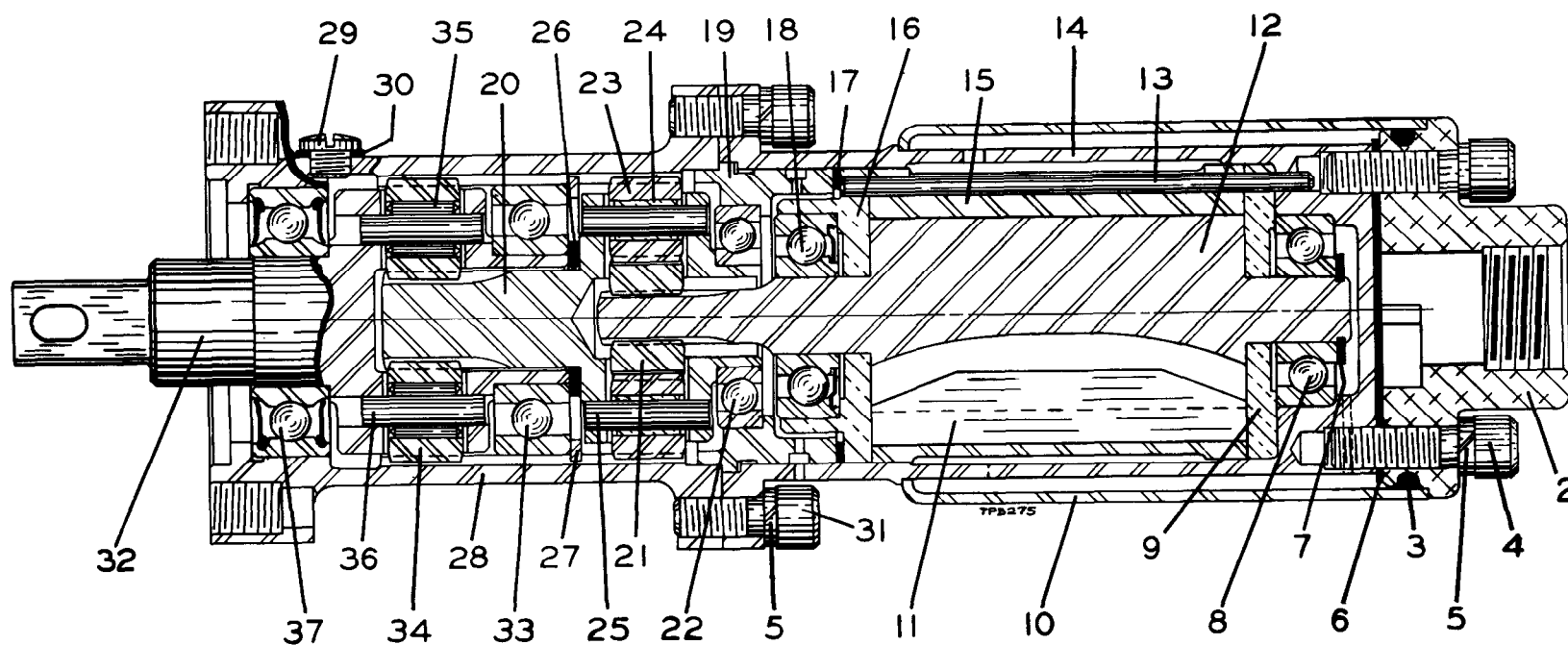
BACK HEAD USED ON REVERSIBLE MOTORS
