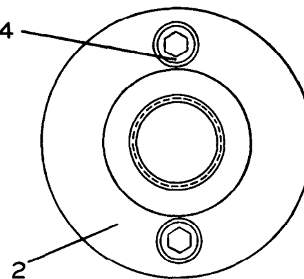
BACK HEAD USED ON NON-REVERSIBLE MOTORS
