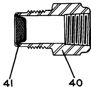
AIR STRAINER
